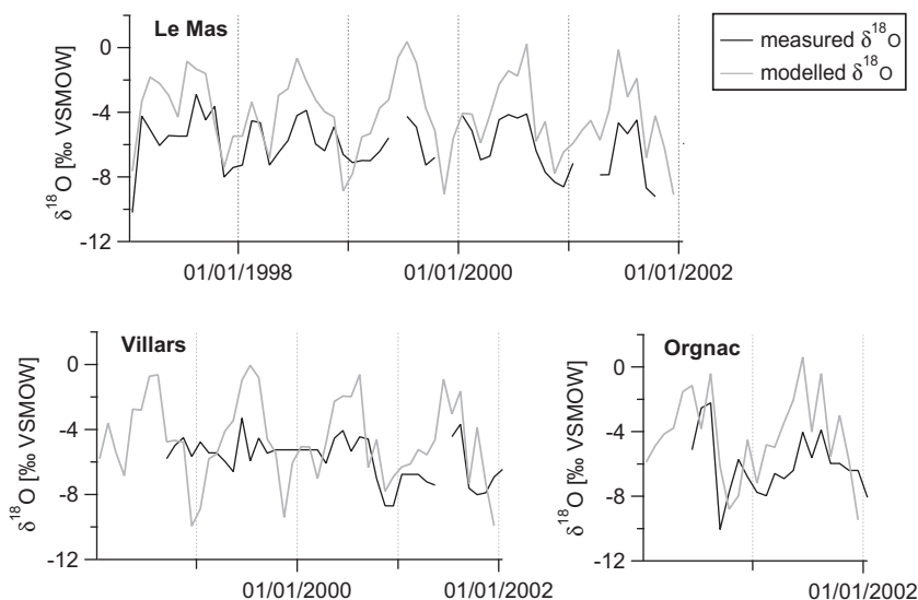
Fig. 9. Comparison between measured precipitation \delta^{18}\text{O} (black lines) and REMOiso simulations (grey lines) for Le Mas, Villars, and Orgnac.
