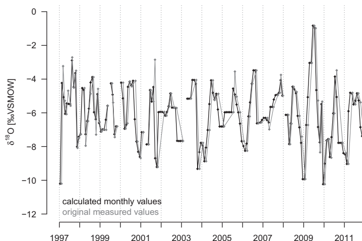
Fig. 3. Comparison between calculated monthly \delta^{18}\text{O} values (in black) and the original measured values (in grey) using the example of Le Mas. The slight shift between the two curves appears because the date assigned to each monthly value is the 15th of that month, whereas the date for the original values is the last day of the sampling period.
