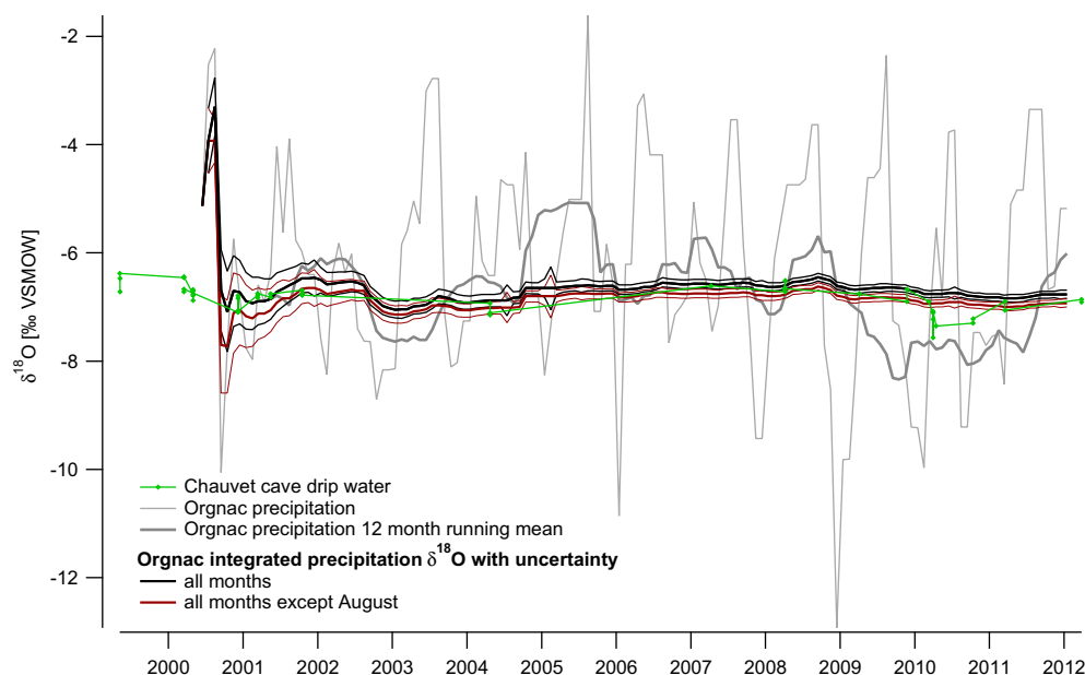
Fig. 11. Precipitation and drip water \delta^{18}\text{O} at Chauvet cave. The thin grey line is the Orgnac precipitation \delta^{18}\text{O} . The green line is the drip water \delta^{18}\text{O} from different stations in Chauvet cave. It is compared to (1) a 12 month running mean of precipitation \delta^{18}\text{O} weighted by the amount of precipitation (it considers all months of the year; thick grey line); (2) the integrated precipitation \delta^{18}\text{O} for all months (black) and for all months except August (brown) with their respective uncertainties. (For interpretation of the references to colour in this figure legend, the reader is referred to the web version of this article.)
